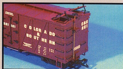
Opening ice hatches and detailed brake wheel including brake platform
